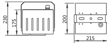
Universal Hanging Bracket
