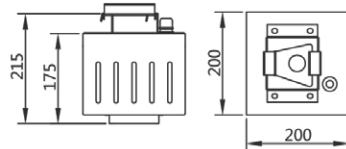
Ceiling Surface Mounting
