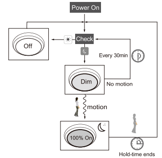
When the natural light level exceeds setpoint off to light, the light will turn off even if when the space is occupied. The light automatically turns on at 10% when natural light is insufficient (no motion).
