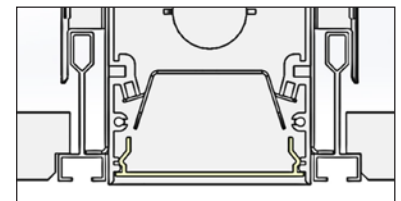
14.29mm (9/16") Slot Grid
