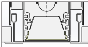
23.81mm (15/16") Grid
