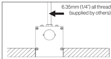
Drywall/Hard Ceiling Trimless
